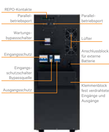
Liebert GXT3-10000T230
